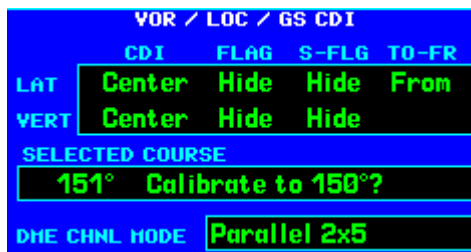
Figure 5-17. VOR/LOC/GS CDI Page
