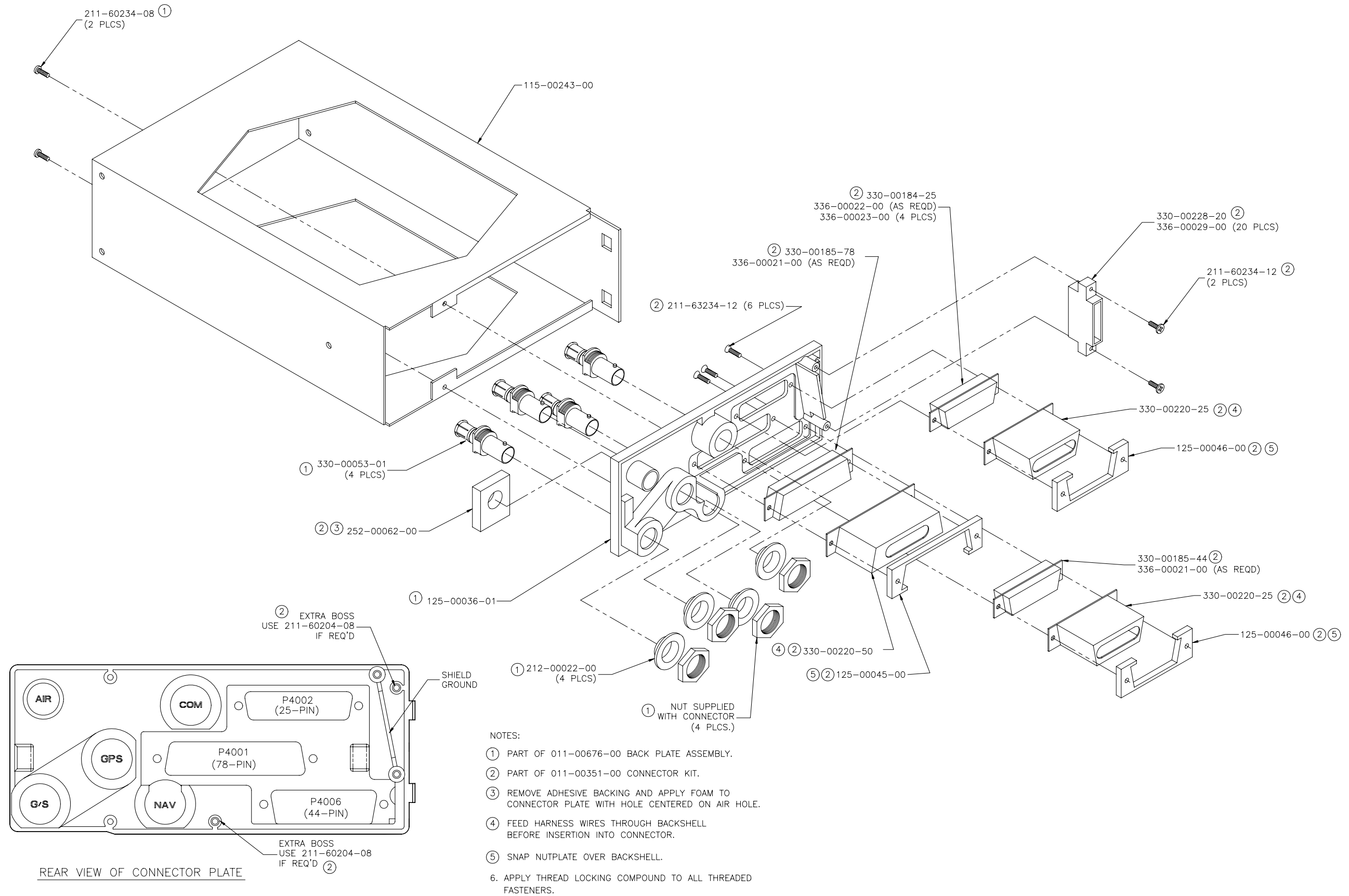
Figure F-5. GNS 430 Mounting Rack Installation
