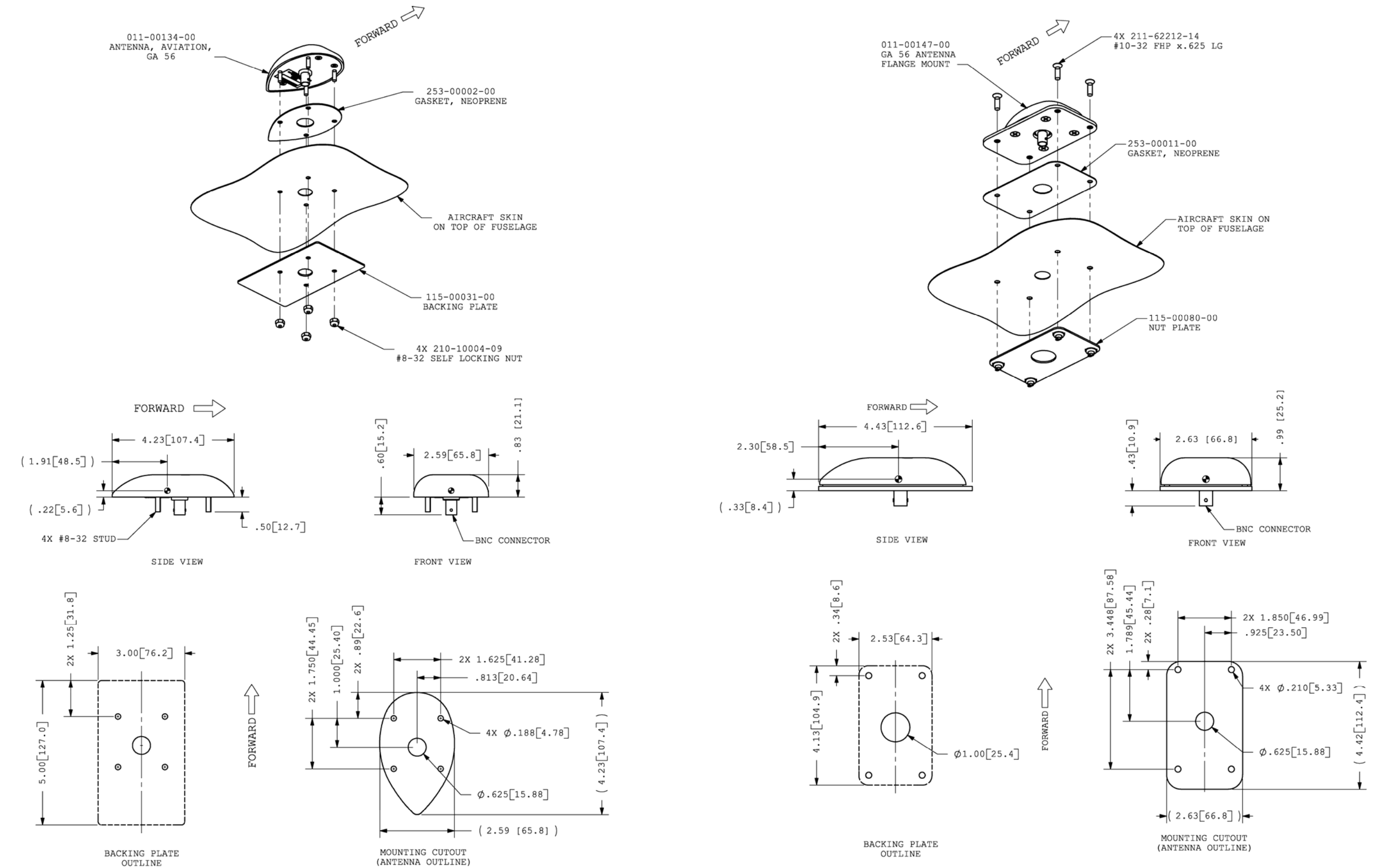
Figure F-1. GA 56 Antenna Installation Drawing
