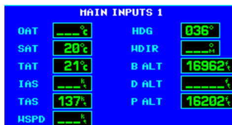
Figure 5-5. MAIN INPUTS 1 Page
