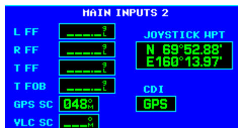
Figure 5-6. MAIN INPUTS 2 Page
