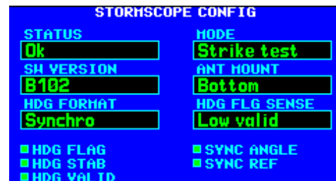
Figure 5-19. STORMSCOPE CONFIG Page
