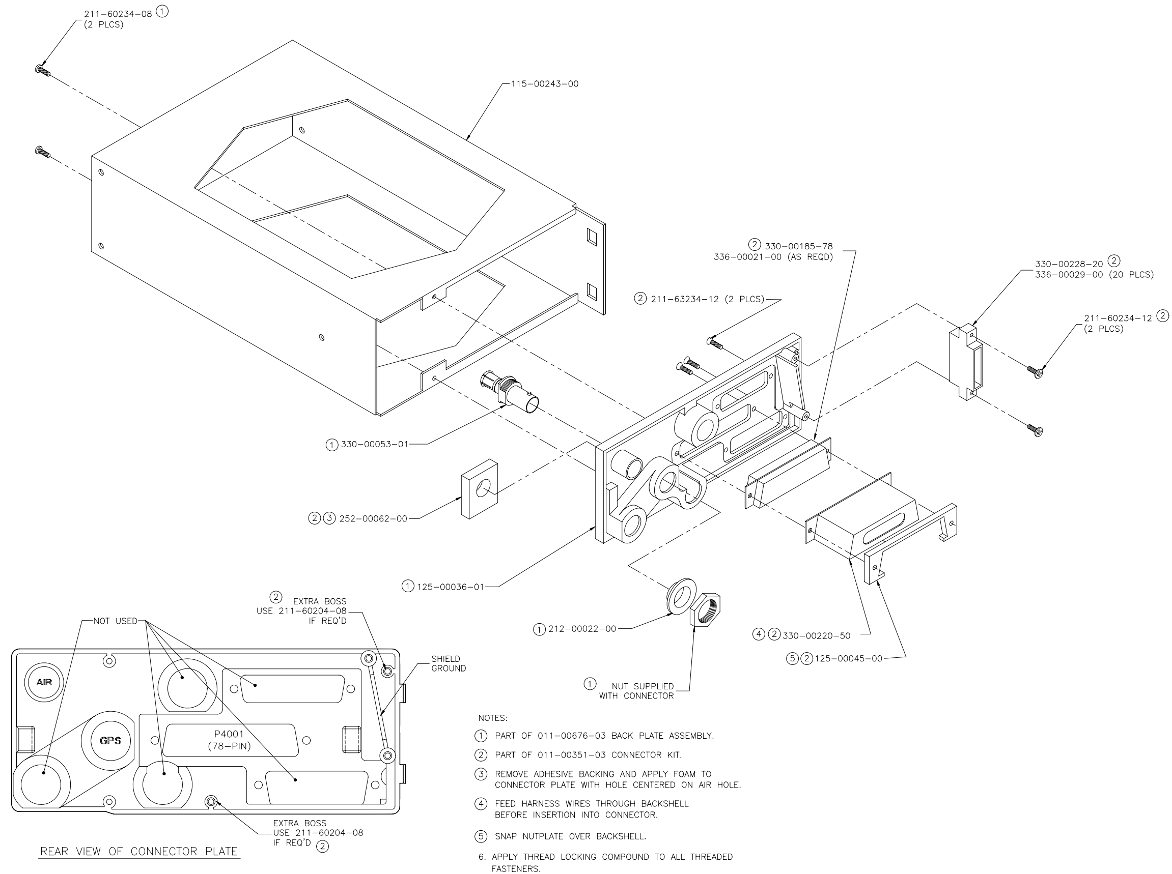
Figure F-7. GPS 400 Mounting Rack Installation
