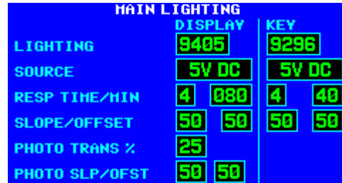
Figure 5-9. MAIN LIGHTING Page (Display Lighting from Lighting Bus)
