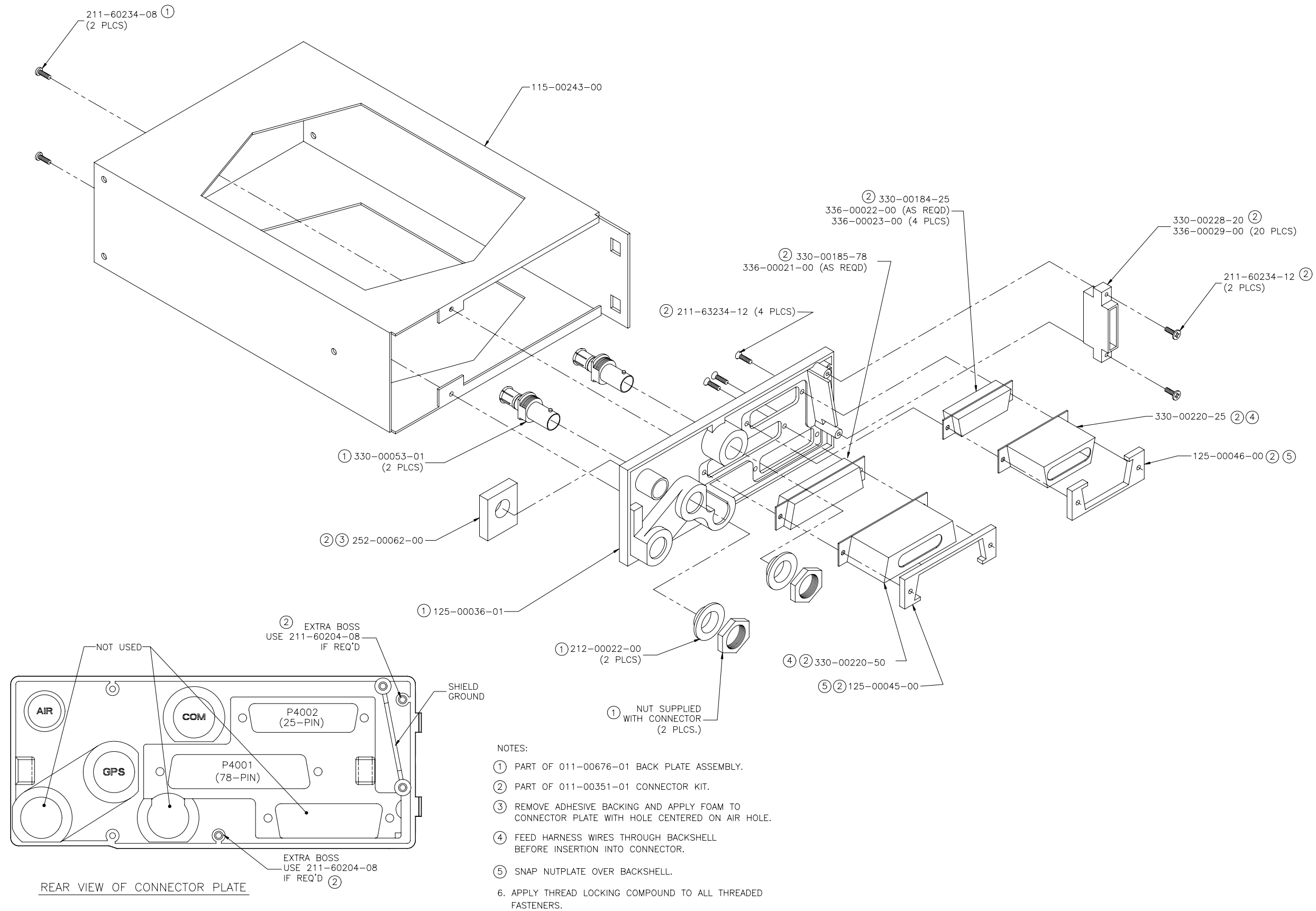
Figure F-6. GNC 420 Mounting Rack Installation
